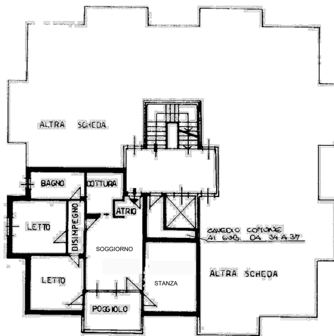
PIANTA PIANO 4 H=260m
